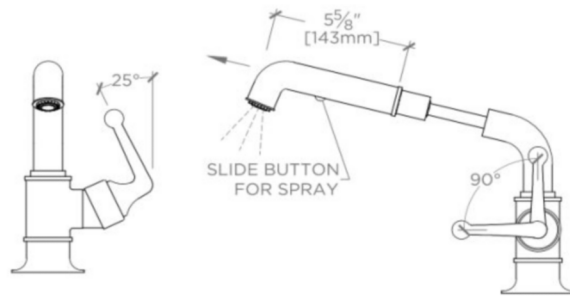
SPRAY PULL OUT VIEW SCALE: 1 1/2"=1'-0"
