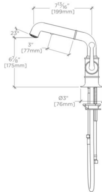
SIDE VIEW SCALE: 1 1/2"=1'-0"
