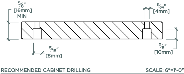
RECOMMENDED CABINET DRILLING
