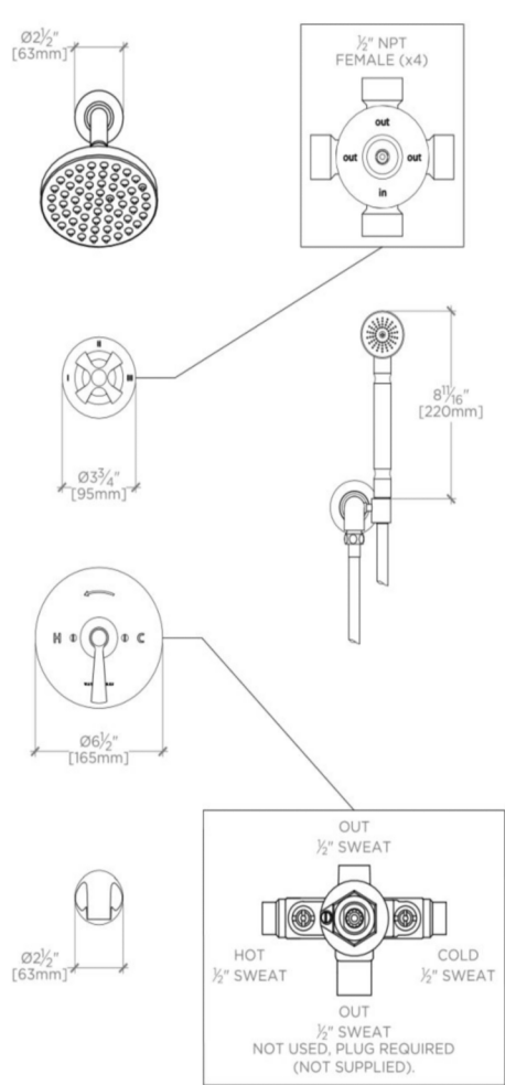
TRSP15 FRONT VIEW
