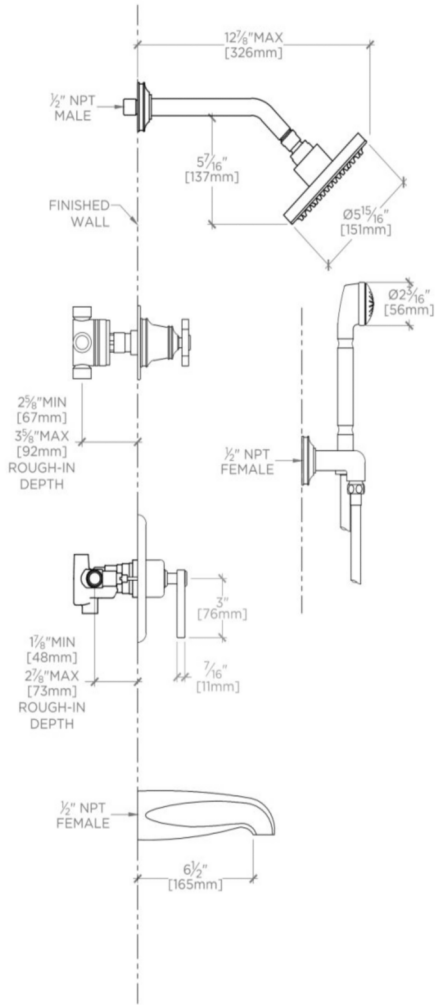
TRSP15 SIDE VIEW
