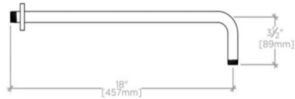
SIDE VIEW SCALE: 1/2"=1'-0"
