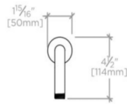
FRONT VIEW SCALE: 1/2"=1'-0"
