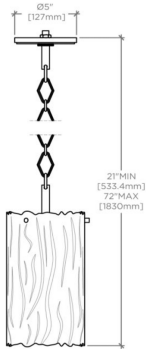
MOUNTING PLATE
