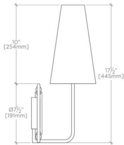
SIDE VIEW SCALE: 1 1/2"=1'-0"
