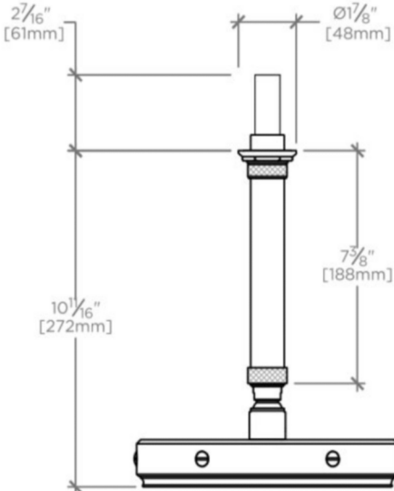
FRONT VIEW SCALE: 2"=1'-0"
