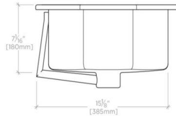
SIDE VIEW SCALE: 1/2"=1'-0"
