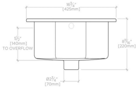
FRONT VIEW SCALE: 1/2"=1'-0"
