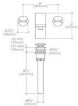
FRONT VIEW SCALE: 1/2"=1'-0"
