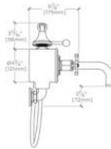
SIDE VIEW SCALE: 5/16"=1'-0"
