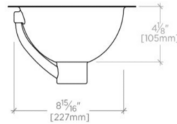
SIDE VIEW SCALE: 1 1/2"=1'-0"
