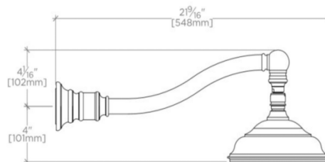
SIDE VIEW SCALE: 1/2"=1'-0"
