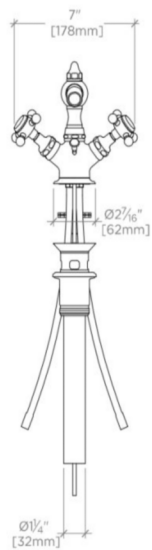
FRONT VIEW SCALE: 1 1/2"=1'-0"
