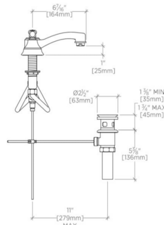
SIDE VIEW SCALE: 1 1/2"=1'-0"
