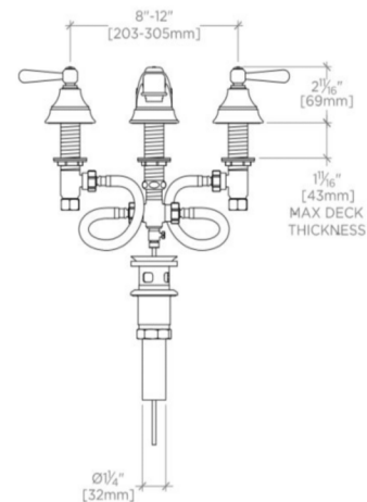
FRONT VIEW SCALE: 1 1/2"=1'-0"
