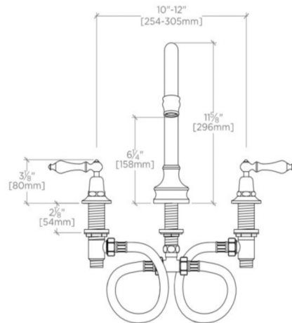
FRONT VIEW SCALE: 1 1/2"=1'-0"
