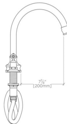
SIDE VIEW SCALE: 1 1/2"=1'-0"
