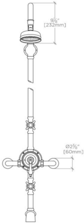
FRONT VIEW SCALE: 1"=1'-0"
