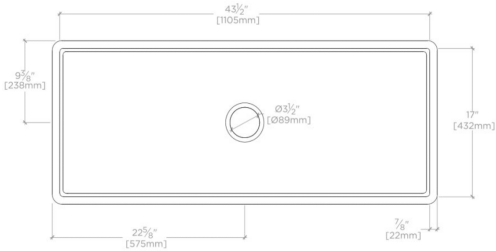
TOP VIEW
