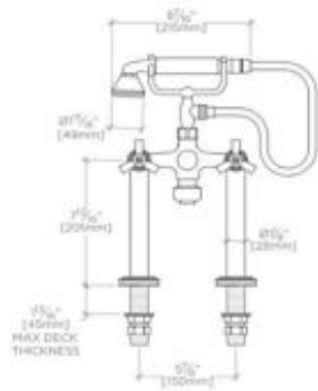
FRONT VIEW SCALE: 5/16"=1'-0"
