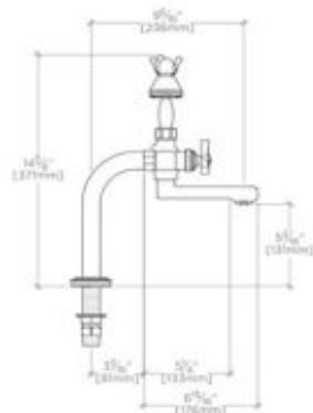
SIDE VIEW SCALE: 5/16"=1'-0"
