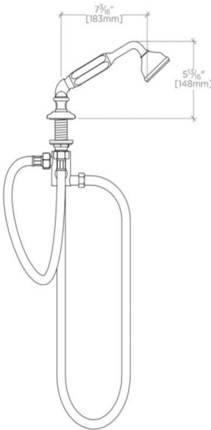
SIDE VIEW SCALE: 1 1/2"=1'-0"
