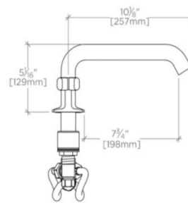
SIDE VIEW SCALE: 1 1/2"=1'-0"
