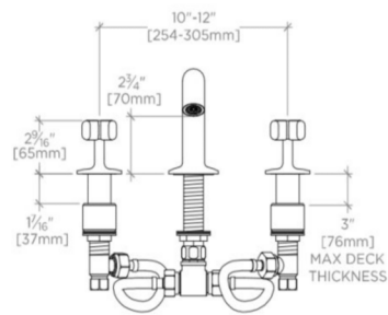
FRONT VIEW SCALE: 1 1/2"=1'-0"
