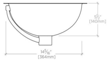
SIDE VIEW SCALE: 1/2"=1'-0"
