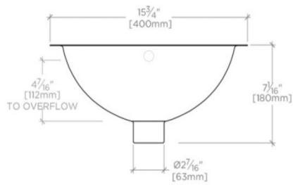
FRONT VIEW SCALE: 1/2"=1'-0"
