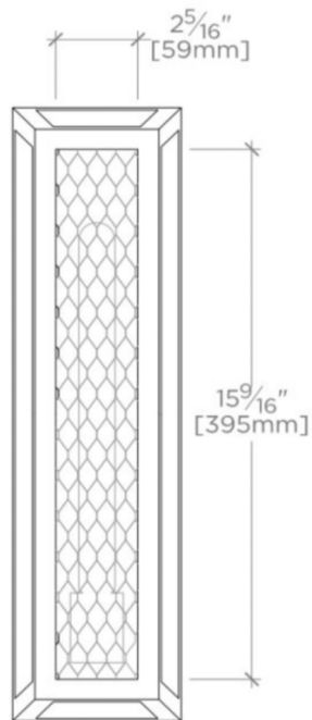
FRONT VIEW SCALE: 2"=1'-0"
