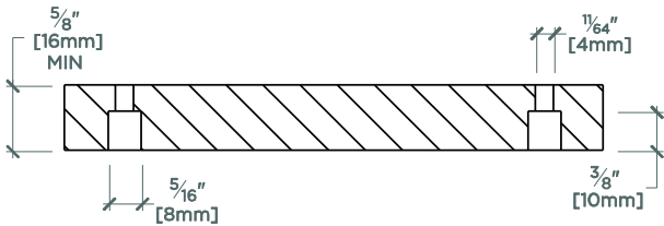
RECOMMENDED CABINET DRILLING SCALE: 6"=1'-0"
