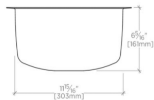
SIDE VIEW SCALE: 1 1/2"=1'-0"
