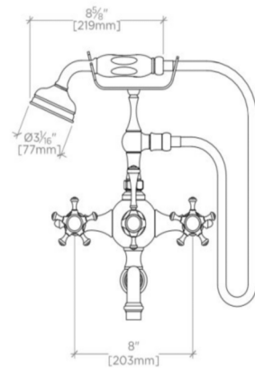
FRONT VIEW SCALE: 1½"=1'-0"
