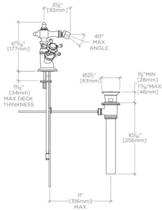
SIDE VIEW SCALE: 1 1/2"=1'-0"
