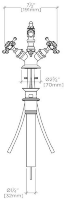
FRONT VIEW SCALE: 1 1/2"=1'-0"
