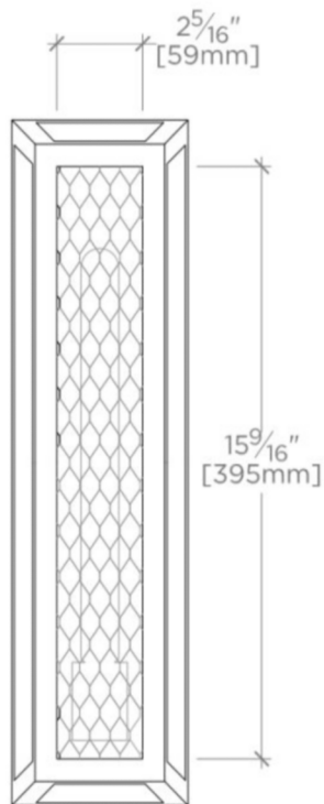
FRONT VIEW SCALE: 2"=1'-0"
